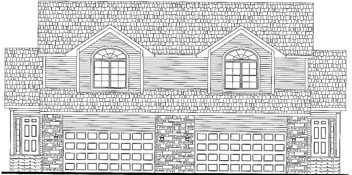
FRONT ELEVATION
